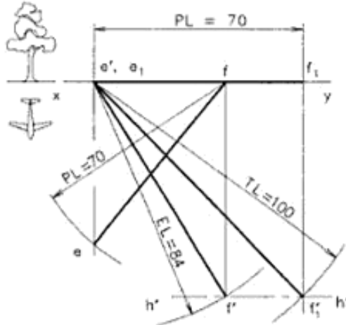
Fig. 10.25 Oblique line in the fourth quadrant.
