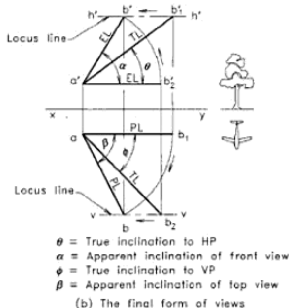
Fig. 10.20 A Line inclined to both the reference planes.
