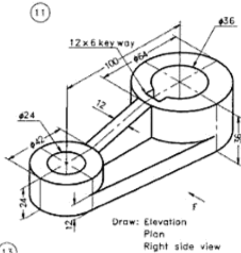
Figure 19.34 A lever.
