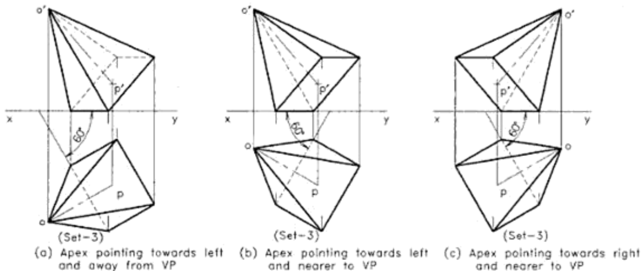
Fig. 12.22 A square pyramid—the three different solutions.
