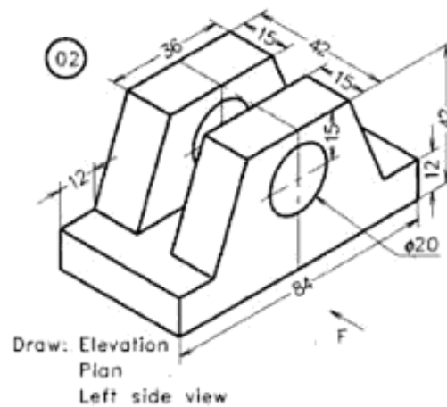
Figure 19.25 A block.
