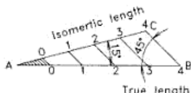
Fig. 16.6 Simplified isometric scale.
