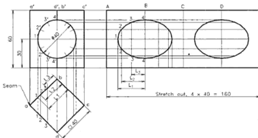
Fig. 15.14 Lateral surface of a prism with a hole.
