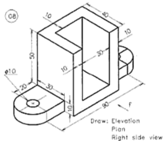
Figure 19.31 Astopper.
