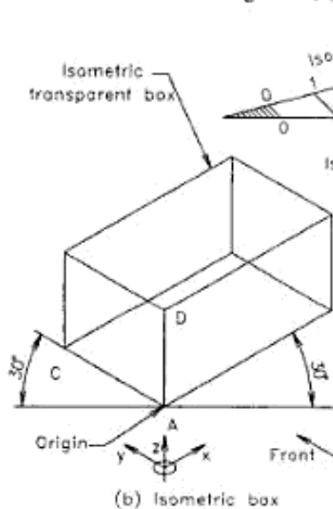
Fig. 16.7 Isometric projection (box method).
