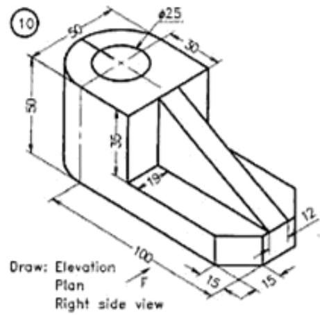
Figure 19.33 A block.
