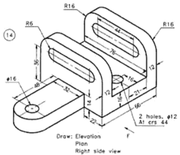
Figure 19.37 A bracket.
