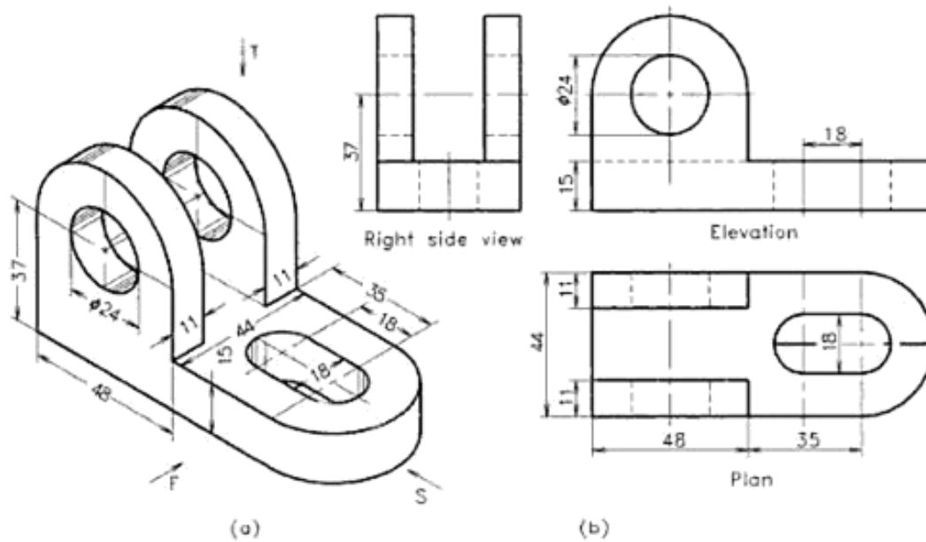
Figure 19.22 Bearing block.
