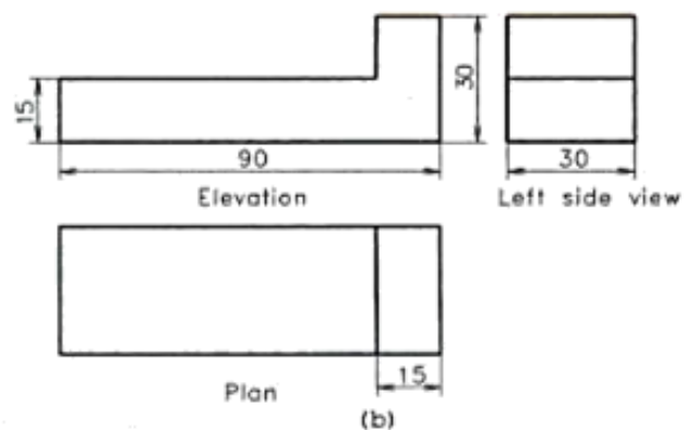
Figure 19.15 Parallel key.
