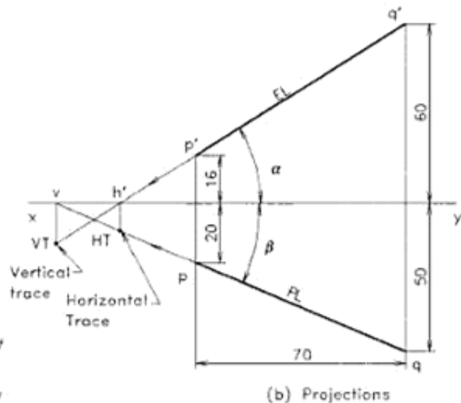
Fig. 10.26 Traces of an oblique line placed in 1st quadrant.
