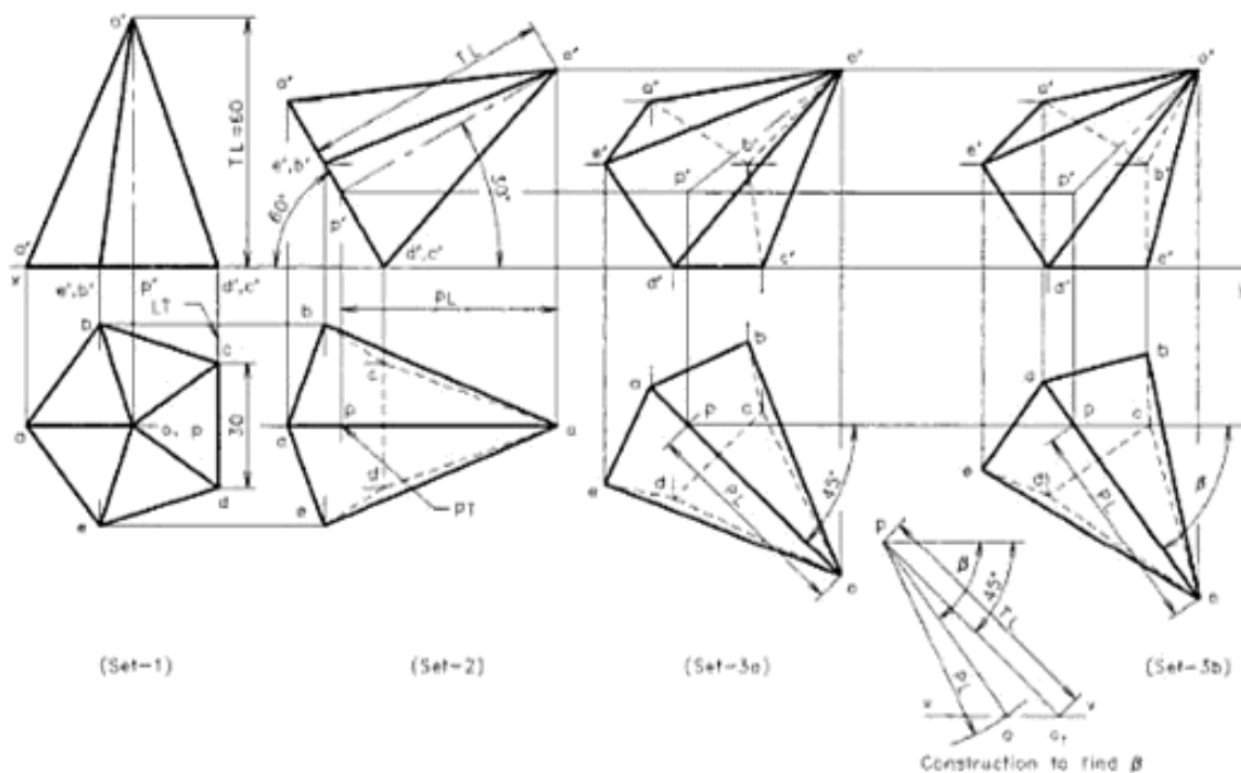
Fig. 12.25 A pentagonal pyramid (axis inclined to both the reference planes).
