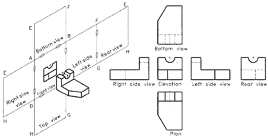
Figure 19.6 Opening of the transparent box (first angle projection).
