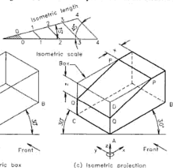
Fig. 16.7 Isometric projection (box method).
