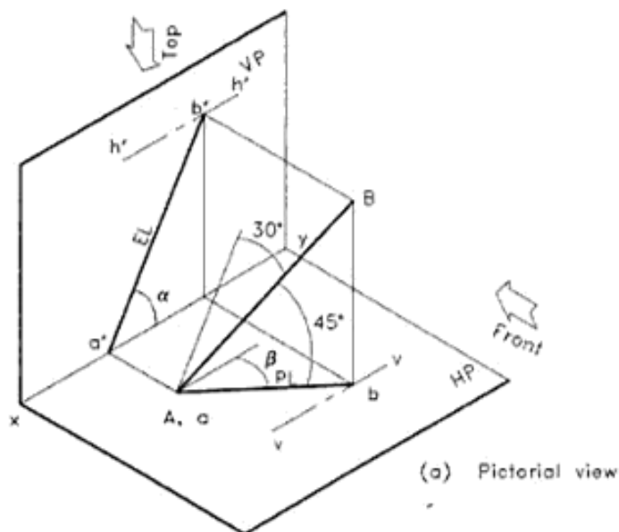
Fig. 10.21 Oblique line in first quadrant.
