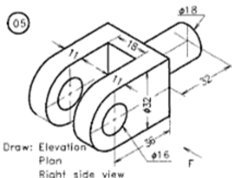
Figure 19.28 Fork end.
