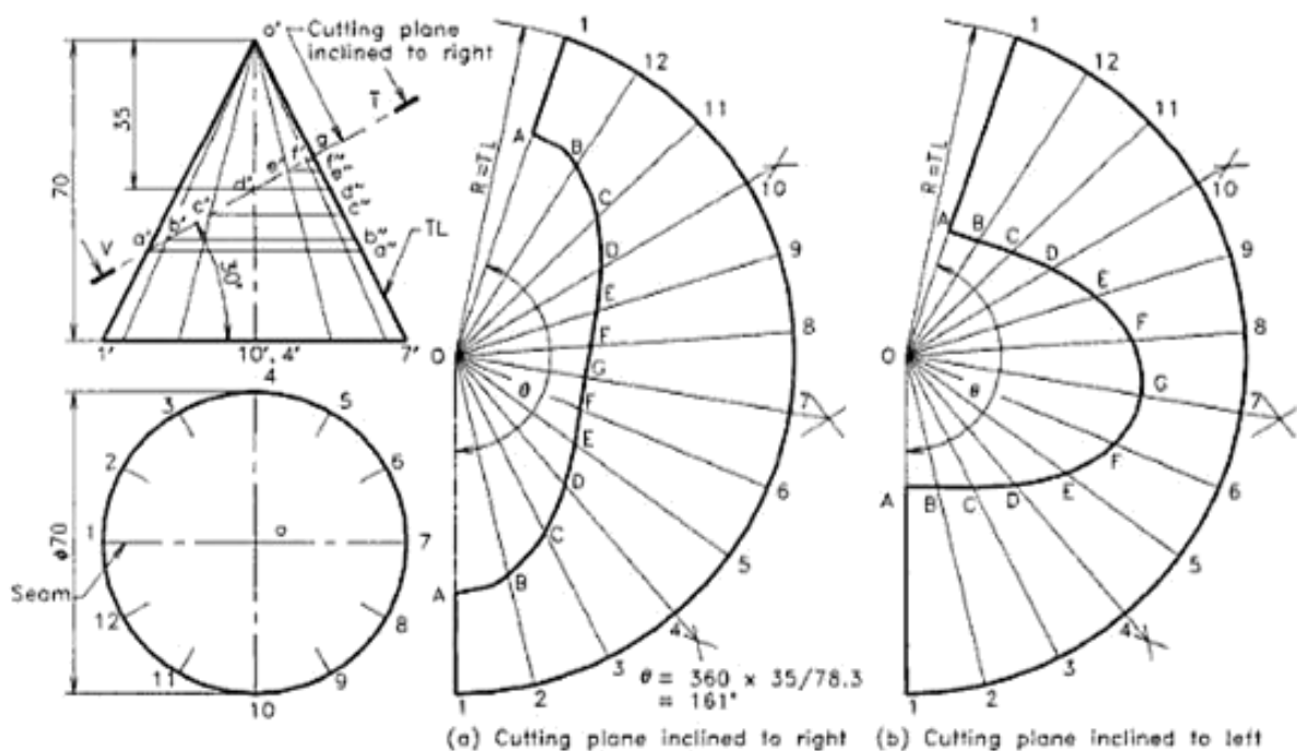
Fig. 15.13 Lateral surface of a truncated cone.
