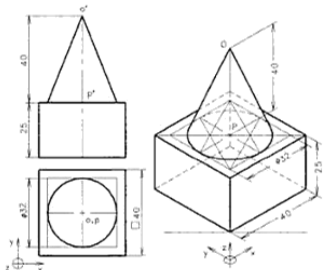
Fig. 16.26 Isometric view (combination of solids).
