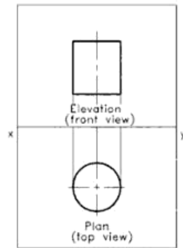
Fig. 9.4 First angle projections of a vertical cylinder.
